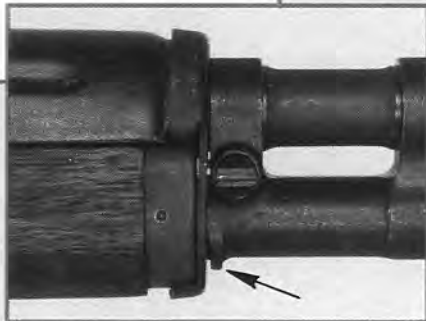
A simple flange at the rear of the gas cylinder stopped the M14's tendency to disassemble itself during Marine bayonet and wire-breaching exercises.
